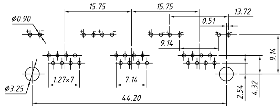
PCB Layout
